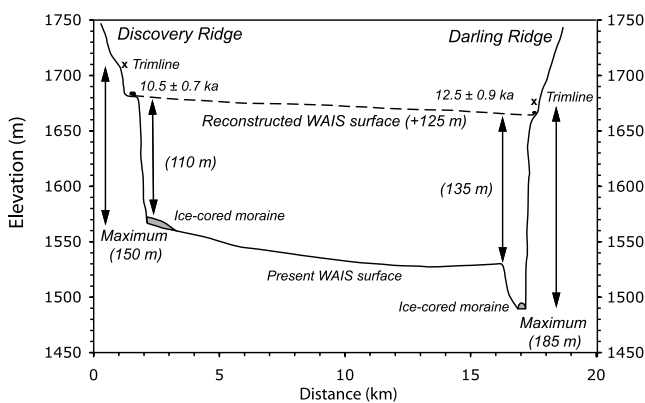
Figure 2. Schematic representation of WAIS elevation changes at the Ohio Range. Vertical exaggeration is 40x. Crosses represent the trimline and filled circles represent glacial erratics. The reconstructed WAIS surface is \sim 125 m above the present day ice surface.
